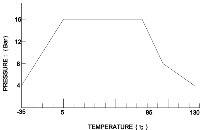
EPDM: PRESSURE/TEMPERATURE GRAPHS
